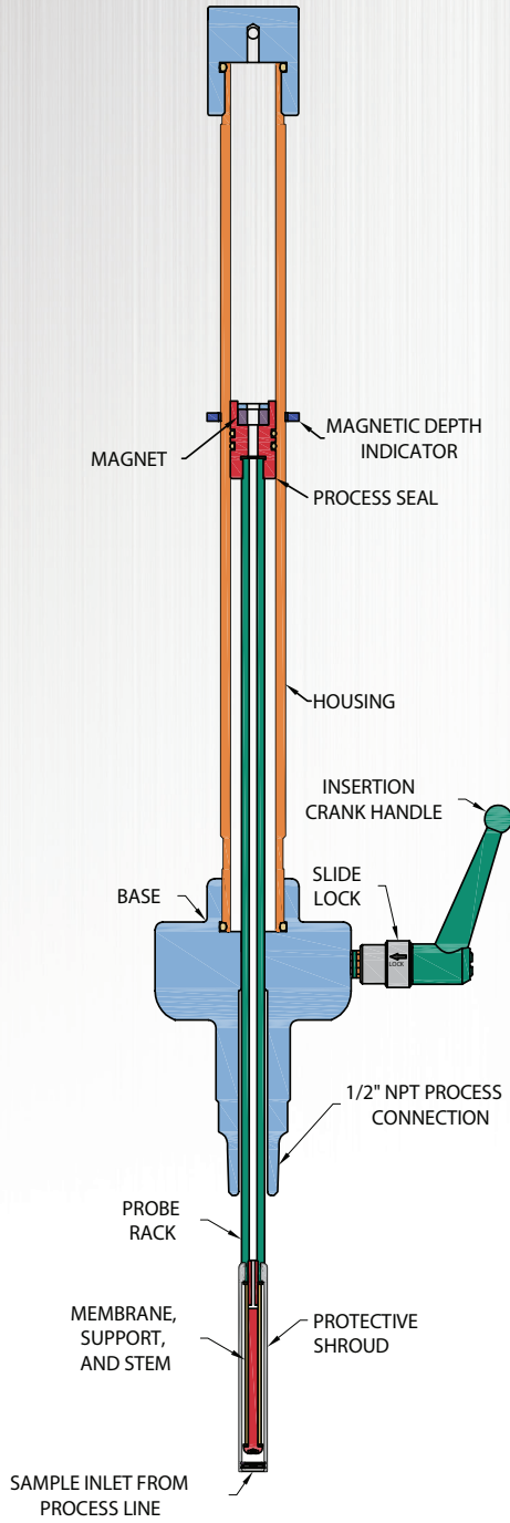
INSERTED VIEW
