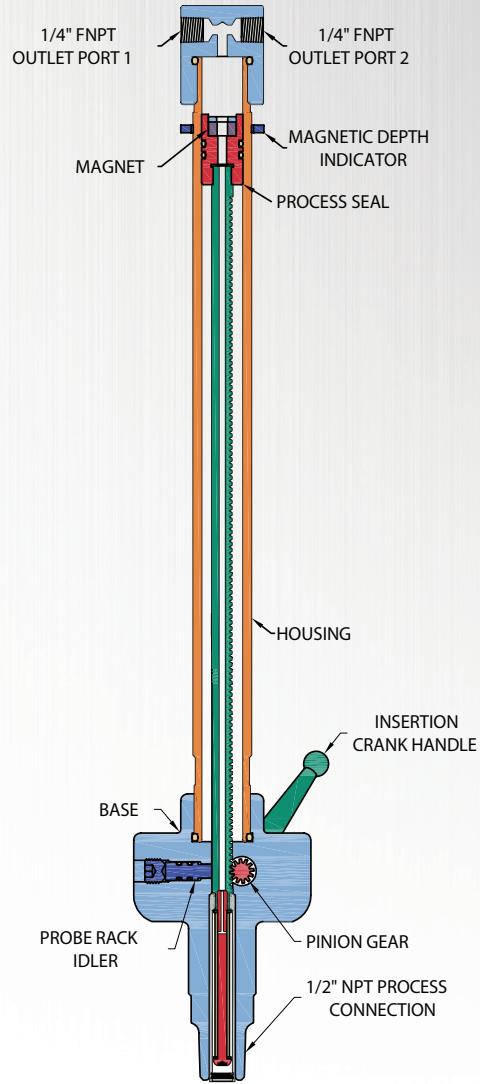
EXTRACTED VIEW
